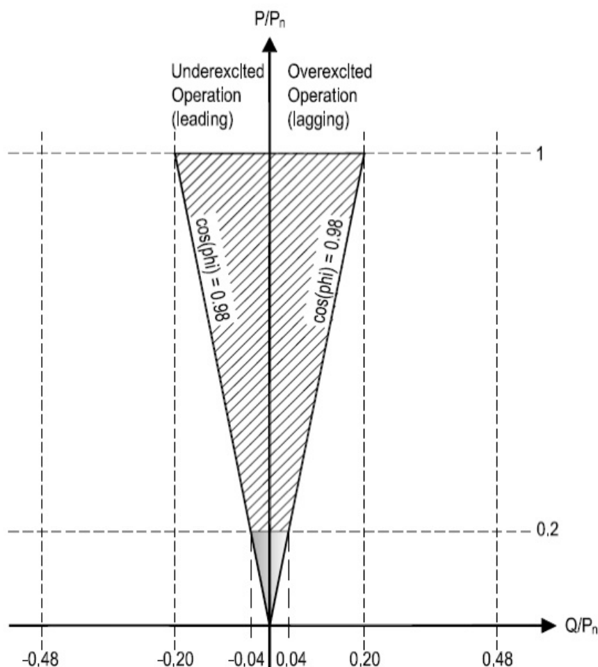
Figure 3 – P-Q capability curve required to a RRGU included in a RRG with P_{MC} < 10 kW
