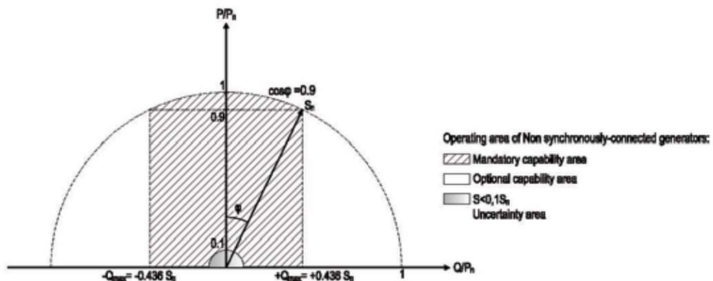
Figure D3- Capability curve for inverters in plants with maximum capacity equal to or larger than 10 kW.
