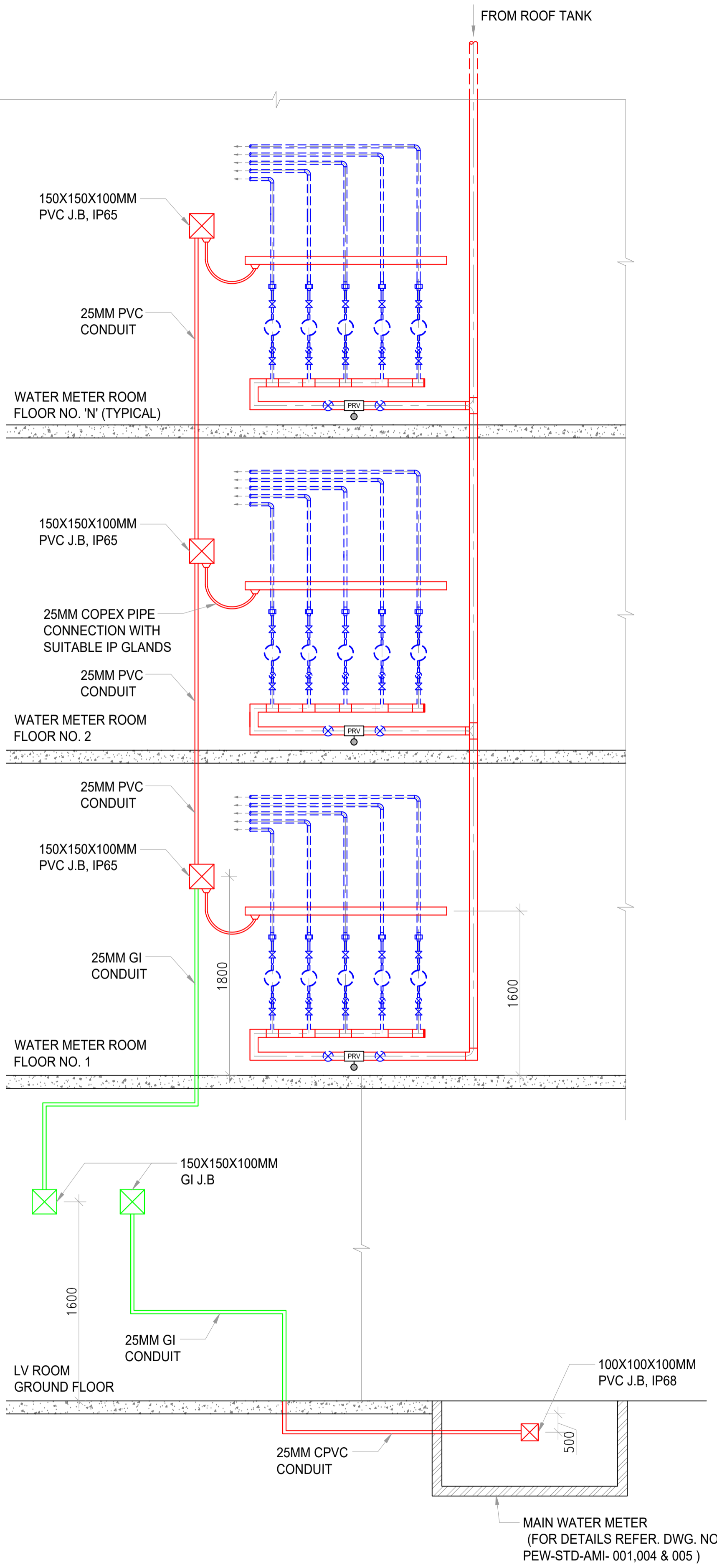
SIDE VIEW
