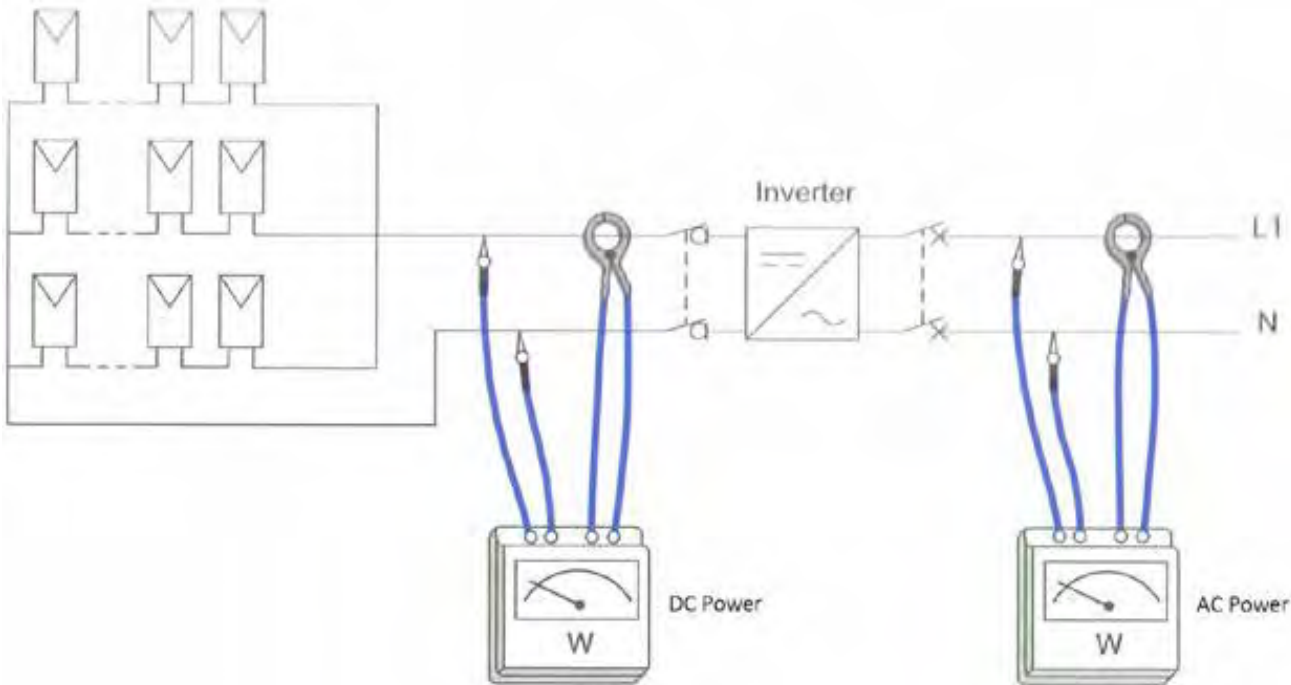
Figure 7 - Power Performance Test. Measurement of DC and AC power on a PV plant
